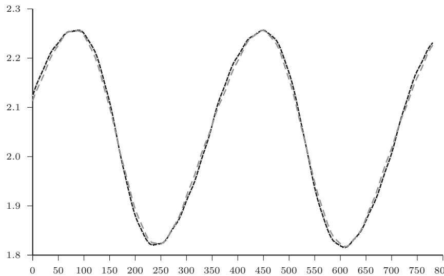
Fig. 2. Difference (1000–1001 C.E.) between siddhāntic and astronomical sidereal solar longitude ( solid black line ) in hours. Dotted white line (atop the black line ) uses the mathematical sine function, rather than an interpolated tabular sine; dashed line uses a fixed epicycle; they are virtually indistinguishable
